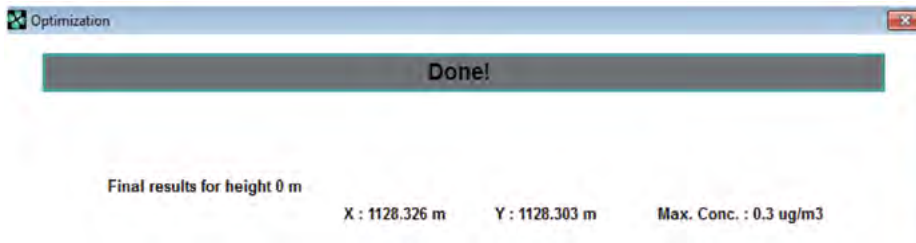
Image 23: Results of maximum concentration for a specific simulation.
