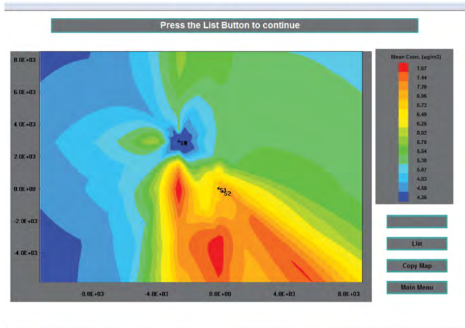
Figure 10a – Isopleths for Spring 1982 with Briggs plume rise and Green dispersion – 43m altitude receptor.
