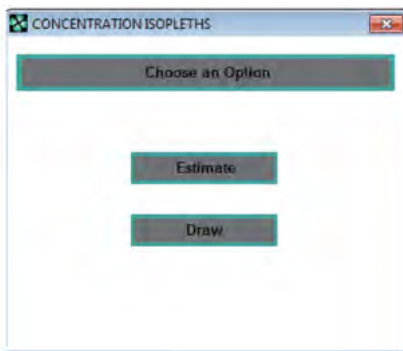
Image 15: Isoleths main menu.
