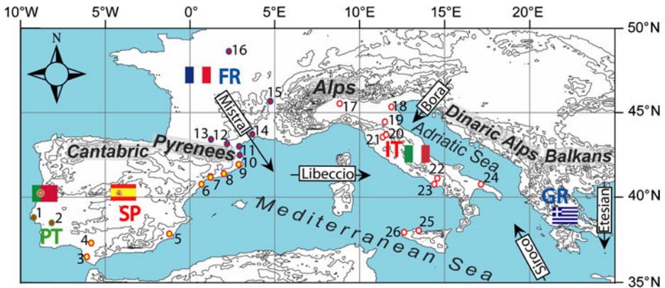
Fig. 1 The Mediterranean Basin with the indicated locations (circles with progressive number label and flag colour code) where documentary proxies and/or instrumental observations have been retrieved for use in this paper, divided by countries: Portugal (PT), Spain (SP), France (FR), Italy (IT) and Greece (GR). The stations are: 1: Lisbon (PT), 2: Évora (PT), 3: Cadiz (SP), 4: Seville (SP), 5: Murcia (SP), 6: Tortosa (SP), 7: Tarragona (SP), 8: Barcelona (SP), 9: Girona (SP), 10: Perpignan (FR), 11: Narbonne (FR), 12: Carcassonne (FR), 13: Toulouse (FR), 14: Montpellier (FR), 15: Lyon (FR), 16: Paris (FR), 17: Milan (IT), 18: Padua (IT), 19: Bologna (IT), 20: Vallombrosa (IT), 21: Florence (IT), 22: Benevento (IT), 23: Naples (IT), 24: Locorotondo, 25: Palermo (IT) and 26: Erice (IT)
